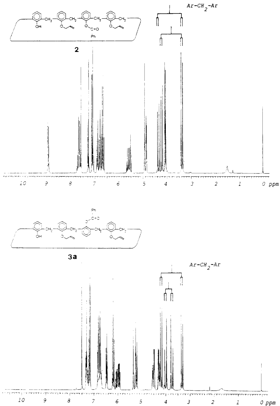
Figure 1. The 1 H-NMR spectra of 1,3-diallyloxy-2-benzoyloxy-calix[4]arenes 2 and 3a .
